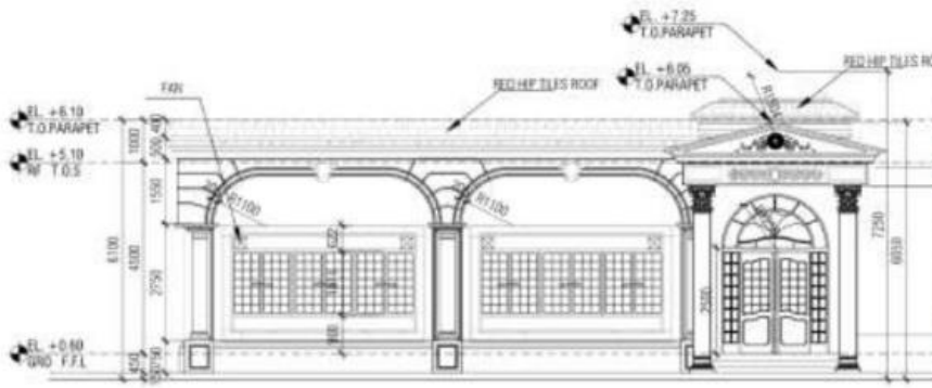
MAIN ELEVATION
