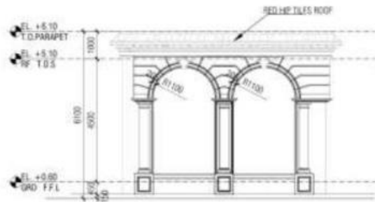
SIDE ELEVATION
